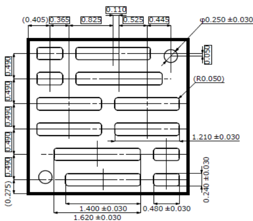
(Reference) Board Land and Stencil Mask Pattern
